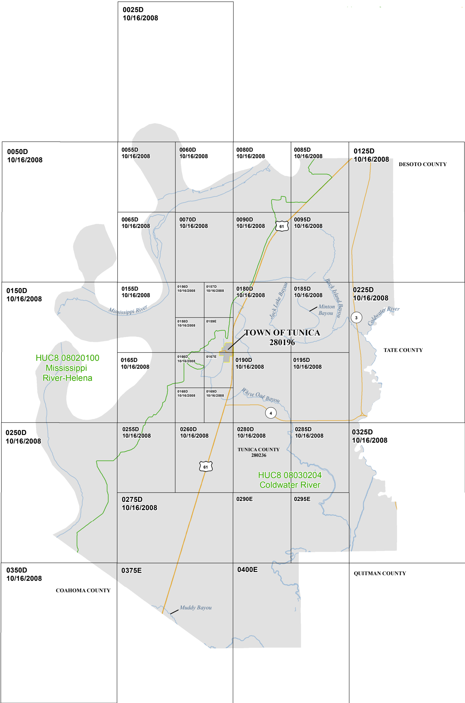
Figure 1: FIRM Index
